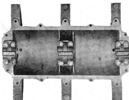
LOWER HALF OF CRANK CASE.
